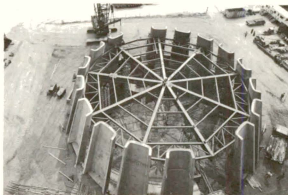
An accelerated schedule over the Memorial Day weekend brought auditorium construction to this state of completion.
